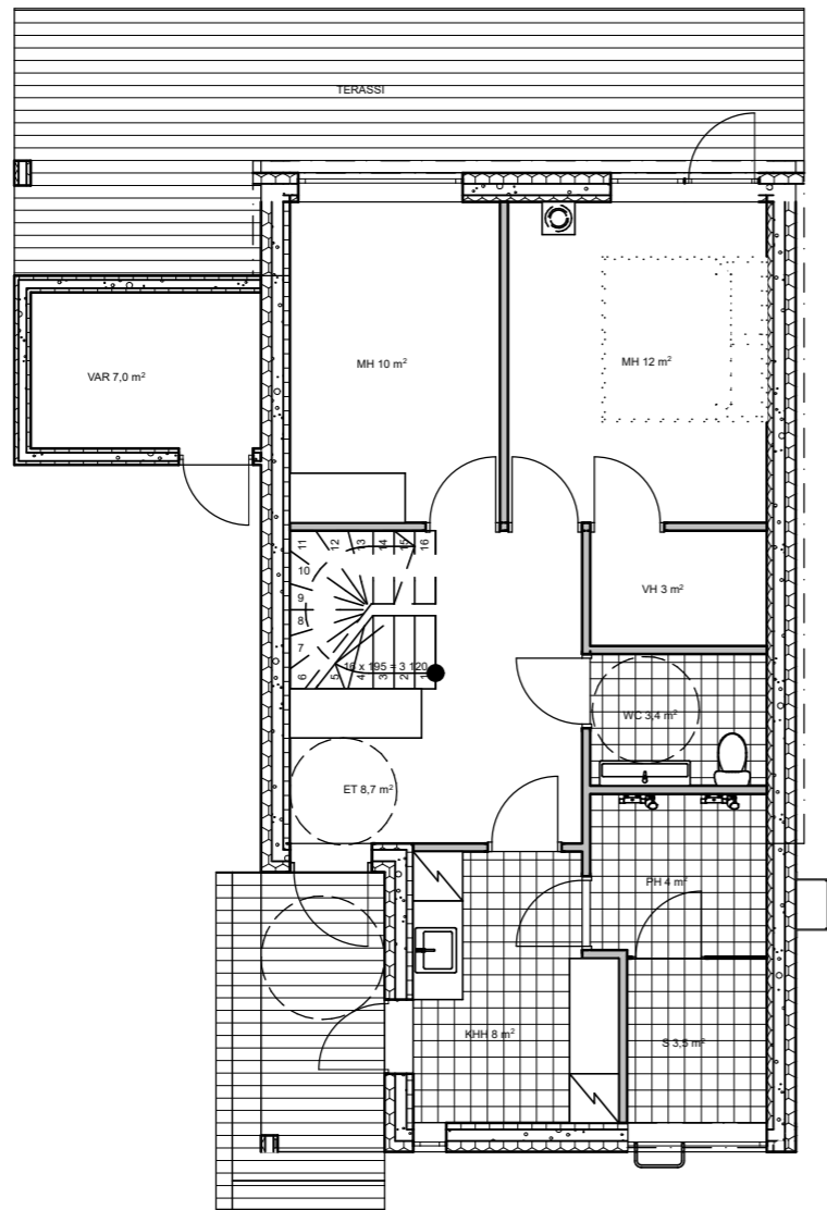
1.krs
